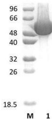
Figure 1. SDS-PAGE analysis of ZgPgx28A (GH28) was conducted in (Lane 1), employing a 14% polyacrylamide gel. The enzyme exhibits a band corresponding to a molecular weight of approximately 49,48 kDa. Lane M contains a Protein Marker for reference.
