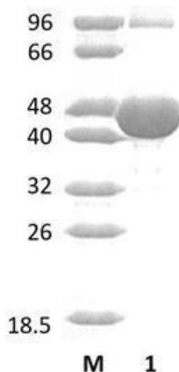
Figure 1. SDS-PAGE analysis of ZgUgl88B (GH88) was conducted in (Lane 1), employing a 14% polyacrylamide gel. The enzyme exhibits a band corresponding to a molecular weight of approximately 45,85 kDa. Lane M contains a Protein Marker for reference.
