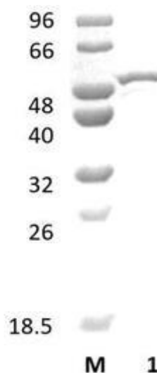
Figure 1. SDS-PAGE analysis of PUlv25A (PL25) was conducted in (Lane 1), employing a 14% polyacrylamide gel. The enzyme exhibits a band corresponding to a molecular weight of approximately 52,14 kDa. Lane M contains a Protein Marker for reference.
