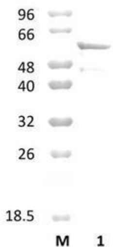
Figure 1. SDS-PAGE analysis of ZgFuc29A (GH29) was conducted in (Lane 1), employing a 14% polyacrylamide gel. The enzyme exhibits a band corresponding to a molecular weight of approximately 56,03 kDa. Lane M contains a Protein Marker for reference.
