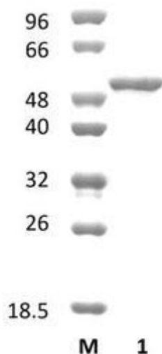
Figure 1. SDS-PAGE analysis of RbPel1A (PL1) was conducted in (Lane 1), employing a 14% polyacrylamide gel. The enzyme exhibits a band corresponding to a molecular weight of approximately 48,70 kDa. Lane M contains a Protein Marker for reference.
