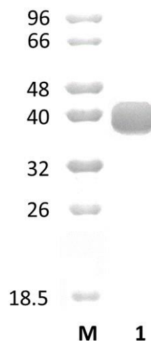
Figure 1. SDS-PAGE analysis of VbNan33A (GH33) was conducted in (Lane 1), employing a 14% polyacrylamide gel. The enzyme exhibits a band corresponding to a molecular weight of approximately 40,24 kDa. Lane M contains a Protein Marker for reference.
