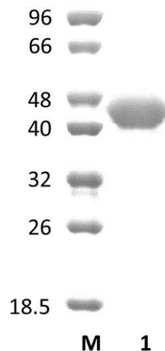
Figure 1. SDS-PAGE analysis of NcAcp20A (GH20) was conducted in (Lane 1), employing a 14% polyacrylamide gel. The enzyme exhibits a band corresponding to a molecular weight of approximately 46,84 kDa. Lane M contains a Protein Marker for reference.
