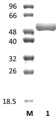
Figure 1. SDS-PAGE analysis of ObNan156A (GH156) was conducted in (Lane 1), employing a 14% polyacrylamide gel. The enzyme exhibits a band corresponding to a molecular weight of approximately 56,42 kDa. Lane M contains a Protein Marker for reference.
