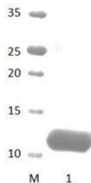
Figure 1. SDS-PAGE analysis of FRMPD2_2 PDZ Domain was conducted in (Lane 1), employing a 14% polyacrylamide gel. The enzyme exhibits a band corresponding to a molecular weight of approximately 12.9 kDa. Lane M contains a Protein Marker for reference.
